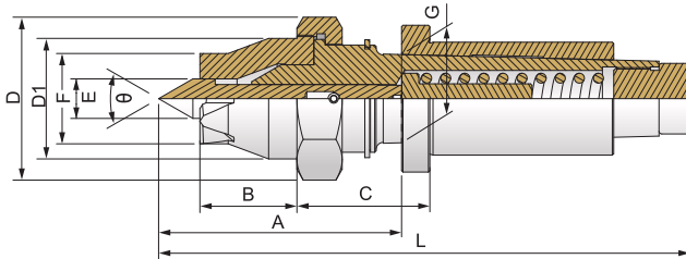
傳動齒+中心針 Driving pins + Centers pins
